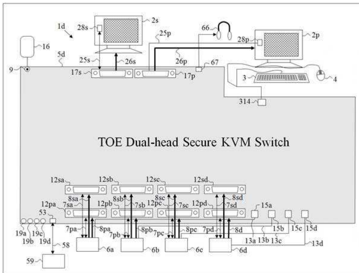
Figure 4 – Dual-Head or Mini-Matrix Secure KVM Switch TOE external interfaces diagram
